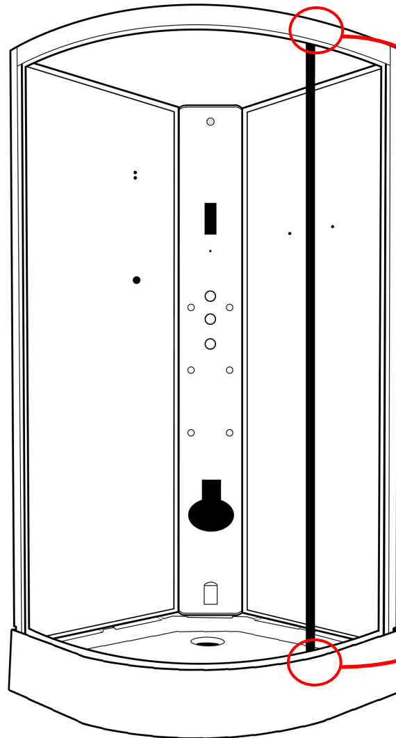
Attach Upright
